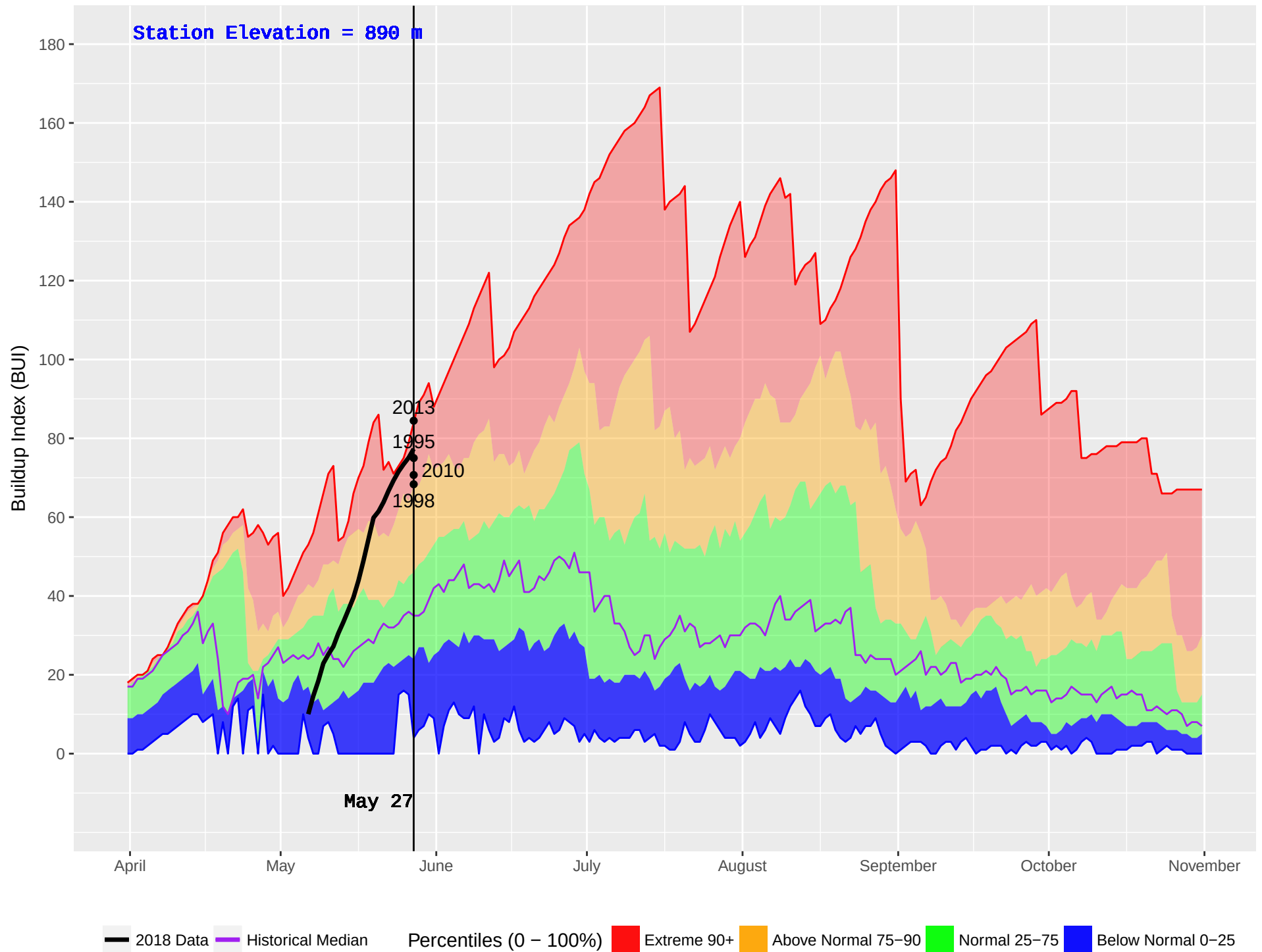
ISKUT (112) : Historical (1979–2016) and Current (2018) Noon Buildup Index (BUI)
