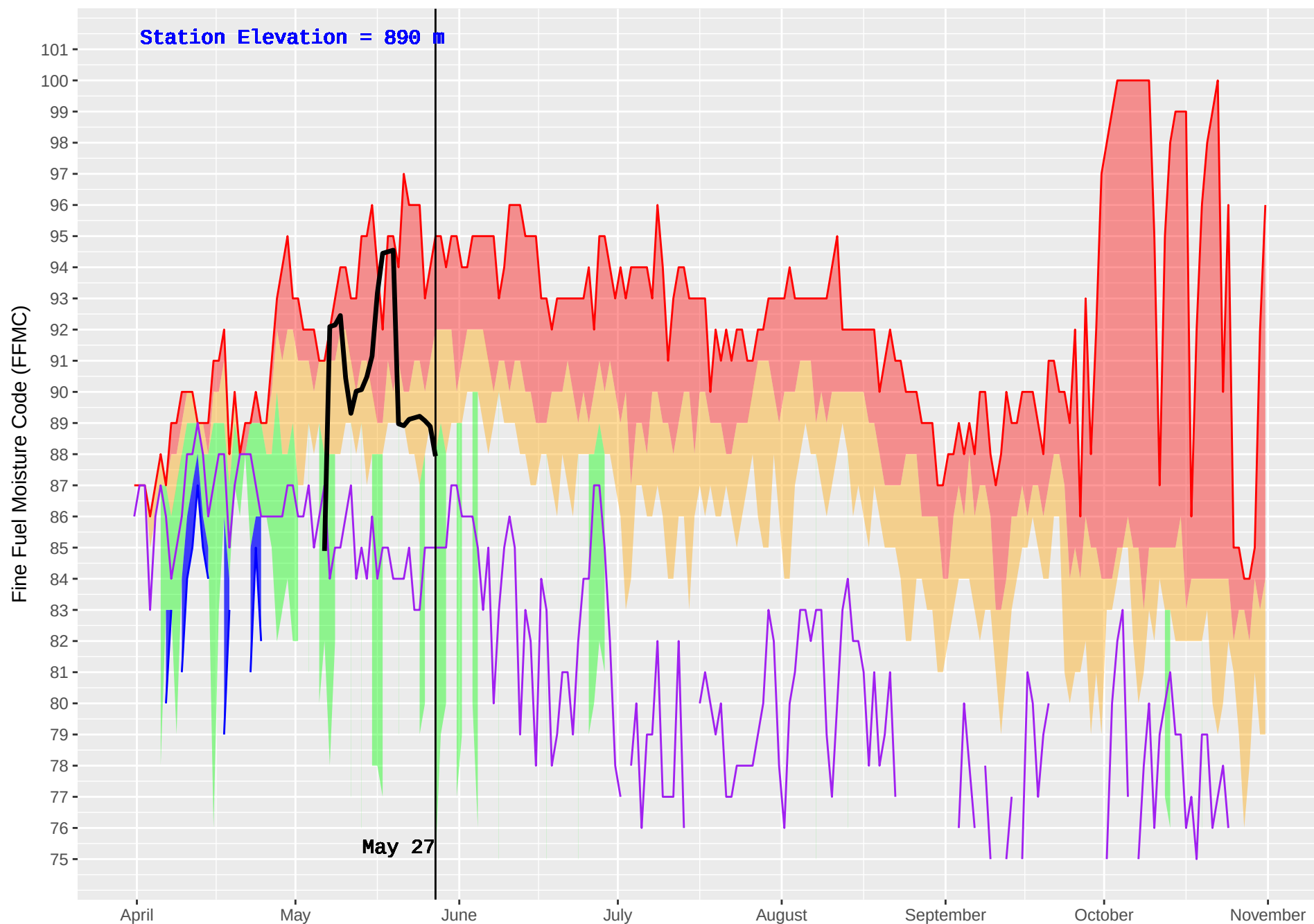
ISKUT (112) : Historical (1979–2016) and Current (2018) Noon Fine Fuel Moisture Code (FFMC)
